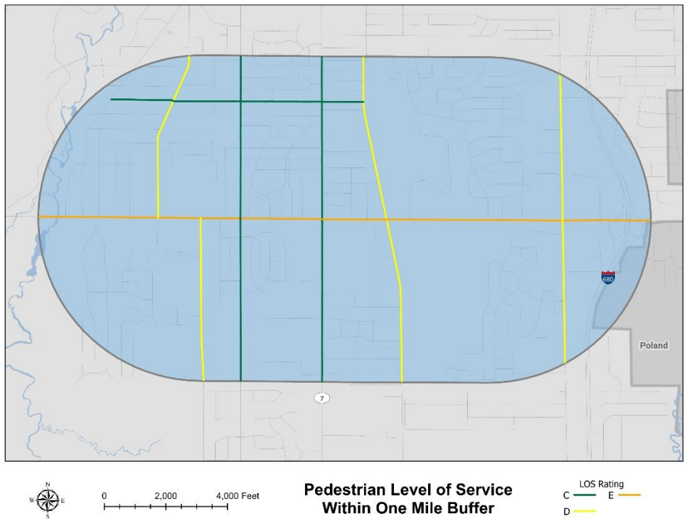
Figure 9: Pedestrian Level of Service ratings for functional class roads within one mile of an activity center in the Boardman area
